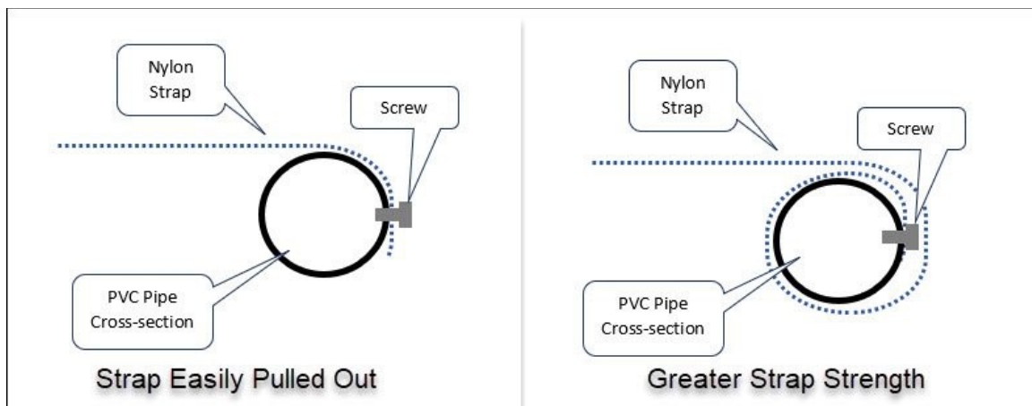
Illustration 1: Comparison of Attaching Nylon Straps
